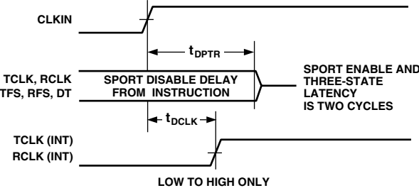
Figure 21. Serial Ports
