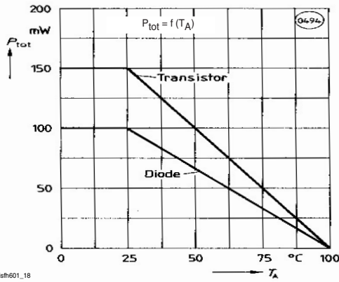
Figure 18. Permissible Power Dissipation for Transistor and Diode
