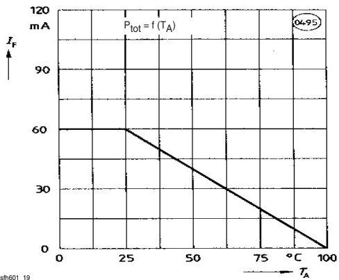
Figure 19. Permissible Forward Current Diode
