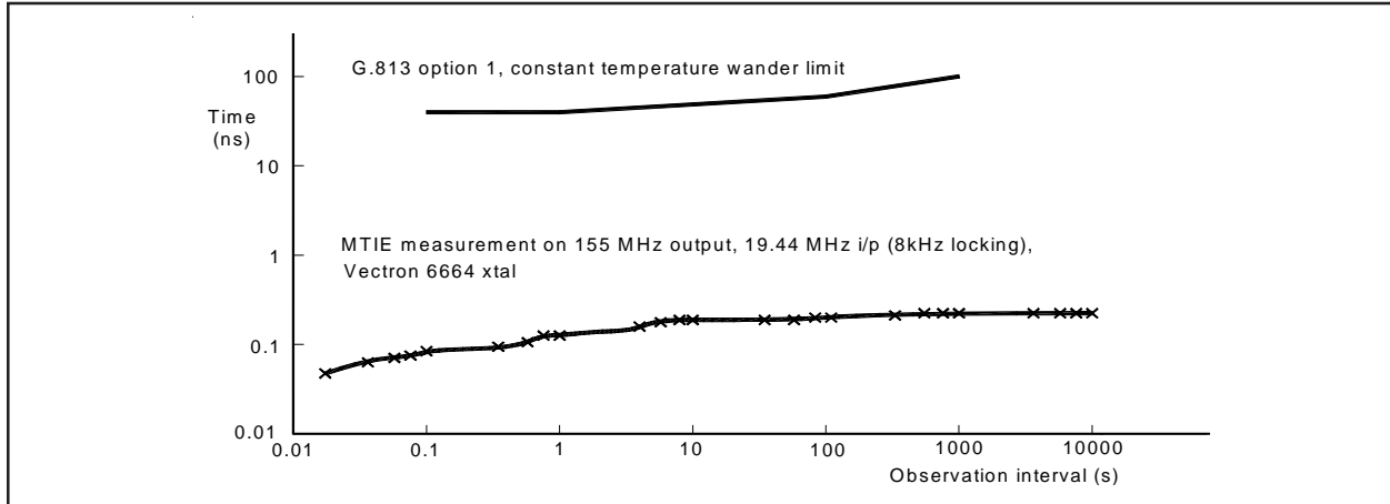
Figure 6. Maximum Time Interval Error of T_{OUTO} Output Port
