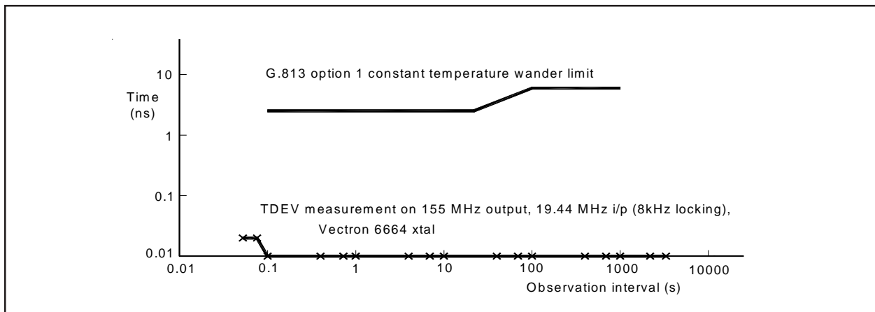
Figure 7. Time Deviation of T_{OUTO} Output Port
