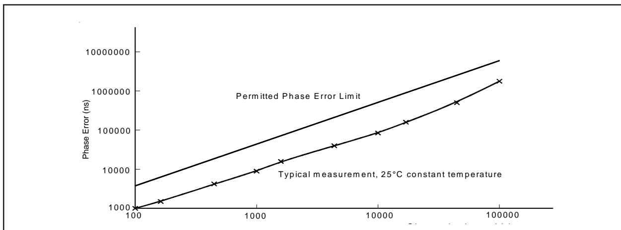
Figure 8. Phase Error Accumulation of T_{OUTO} Output Port in Holdover Mode
