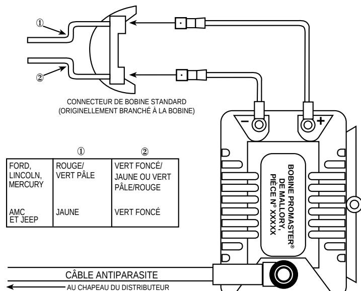
FIGURE 4 ALLUMAGE MOTORCRAFT/DURASPARK FORD, LINCOLN, MERCURY, AMC ET JEEP
