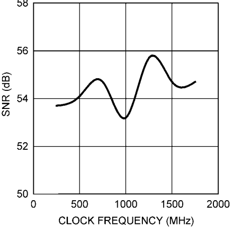
SNR vs. CLOCK FREQUENCY (ADC10D1500)
