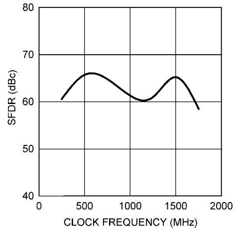
SFDR vs. CLOCK FREQUENCY (ADC10D1500)
