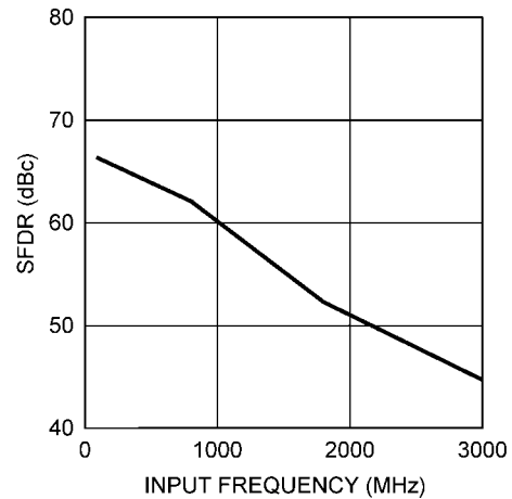
SFDR vs. INPUT FREQUENCY (ADC10D1500)
