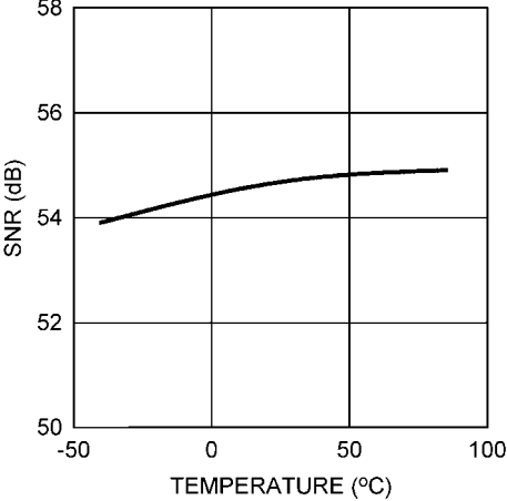
SNR vs. TEMPERATURE (ADC10D1500)
