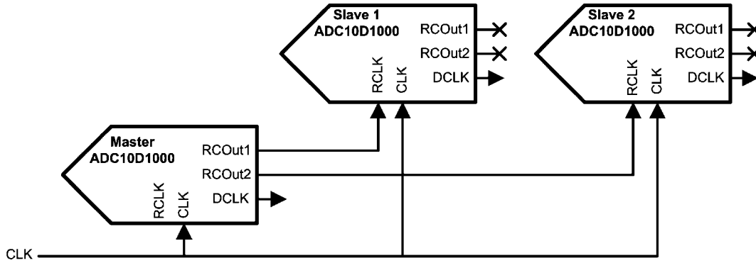
FIGURE 19. AutoSync Example
