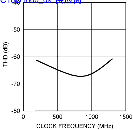
THD vs. CLOCK FREQUENCY (ADC10D1000) 查询"ADC10D1000_09"供应商
