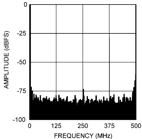
SPECTRAL RESPONSE AT FIN = 498 MHz (ADC10D1000)
