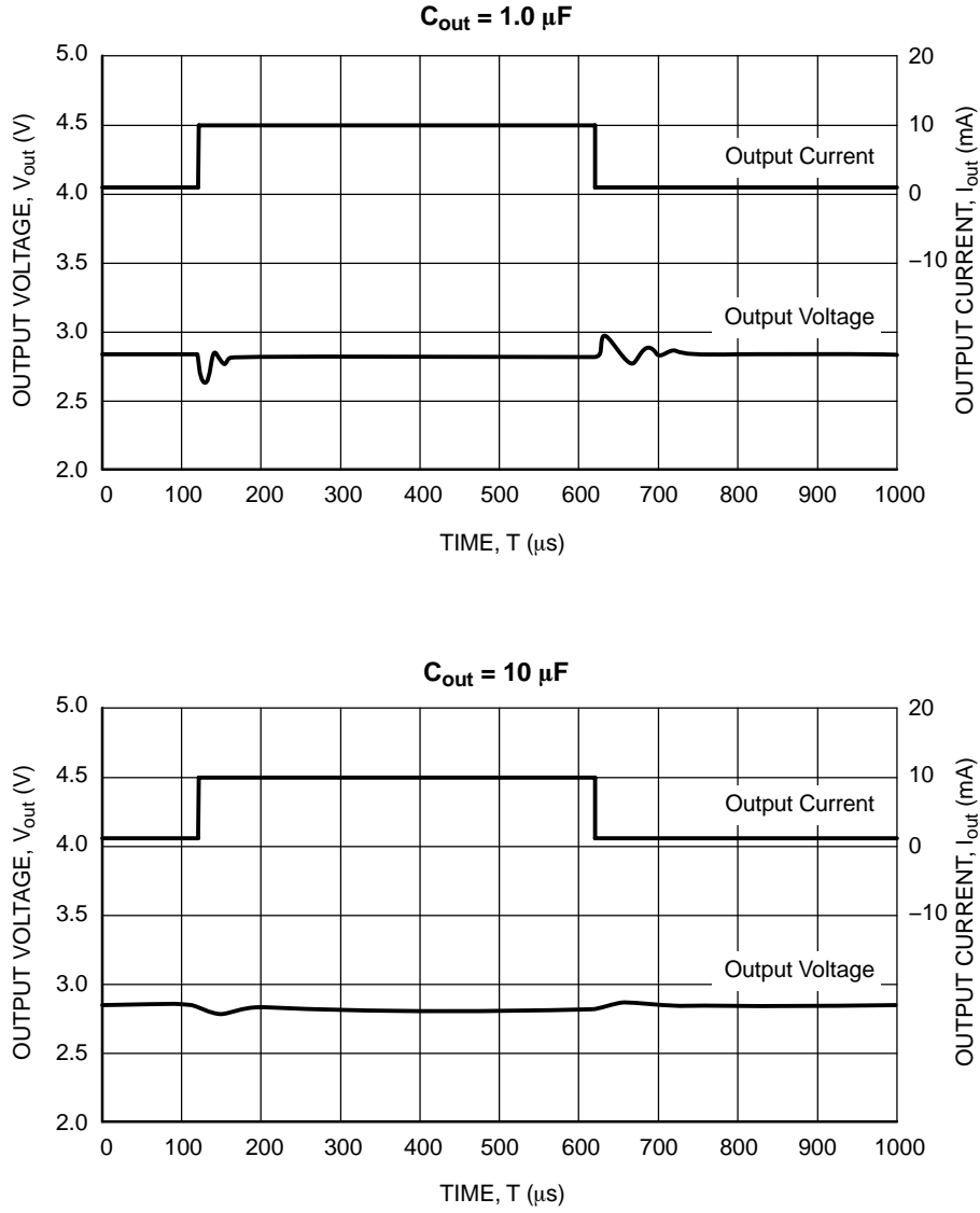
Figure 14. Load Transient Response ( V_{out} = 2.8 \text{ V} , t_r = t_f = 5.0 \mu\text{s} , V_{in} = 3.8 \text{ V} )
