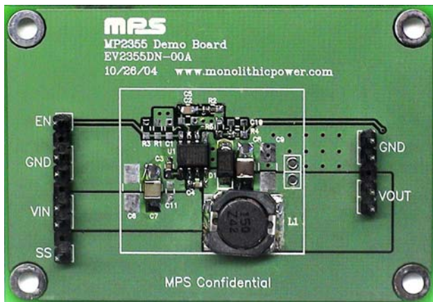
Dimensions (2.6"X x 1.9"Y x 0.4"Z)
