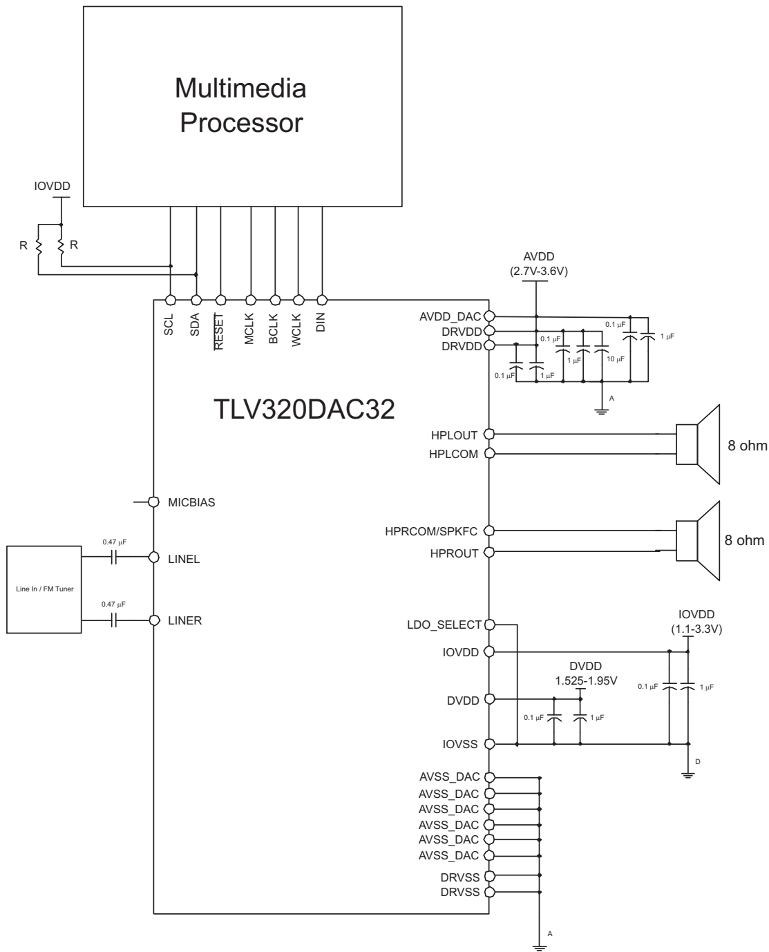
Figure 16. Internal 8-Ω Speaker Driver with External DVDD Supply (LDO Off)
