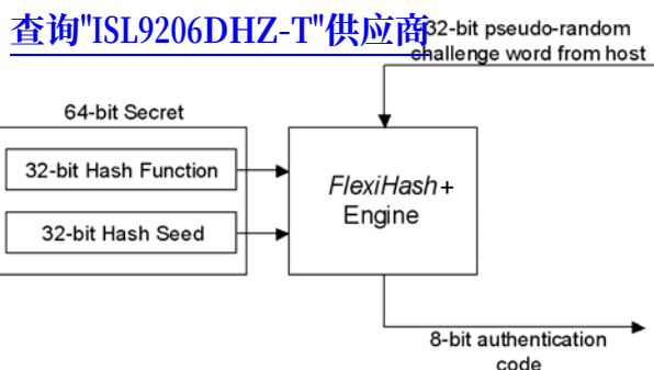
FIGURE 5. AUTHENTICATION PROCESS FLOW DIAGRAM
