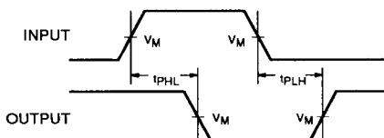
Waveform 1. Propagation Delay For Inverting Output
