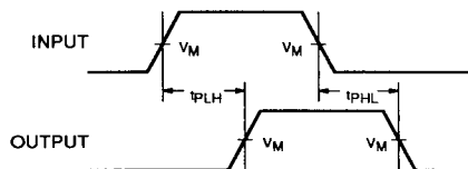
Waveform 2. Propagation Delay For Non-Inverting Output
