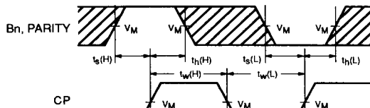
Waveform 6. Data Setup and Hold Times and Clock Pulse Width
