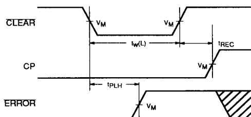
Waveform 5. CLEAR Pulse Width, CLEAR to ERROR Delay and CLEAR to Clock Recovery Time
