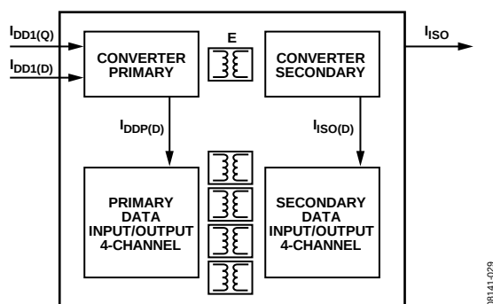
Figure 29. Power Consumption Within the ADuM640x
