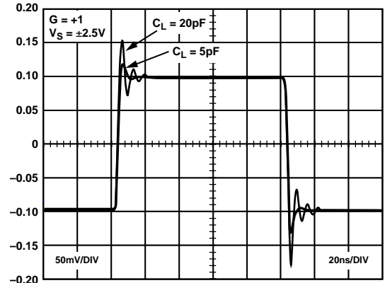
Figure 31. Small Signal Transient Response with Capacitive Load
