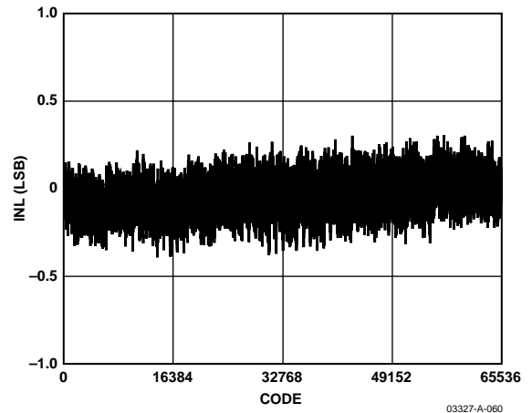
Figure 61. Integral Nonlinearity
