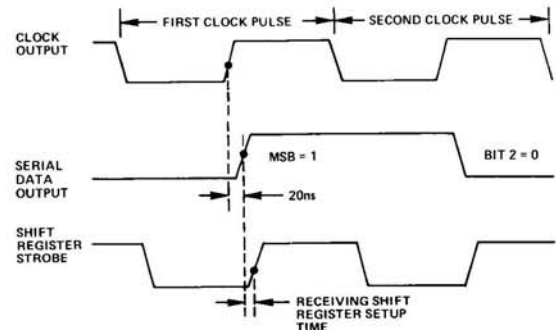
Figure 4. Serial Data Timing Diagram
