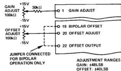
Figure 5. Adjustment Connections
