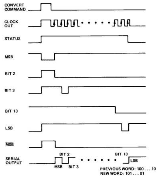
Figure 1. Timing Diagram
