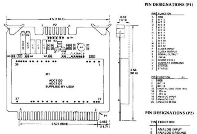
Figure 7. AC1578 Mounting Card
