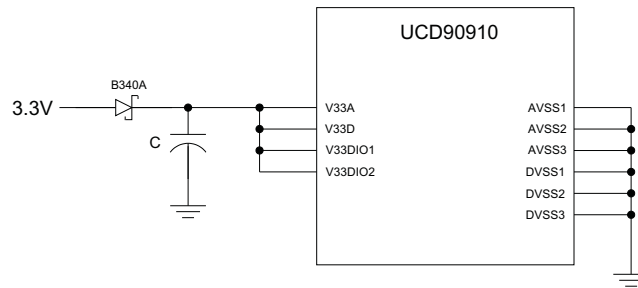
Figure 28. Brownout Circuit
