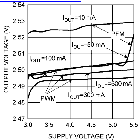
Output Voltage vs. Supply Voltage ( V_{OUT} = 1.5V )
