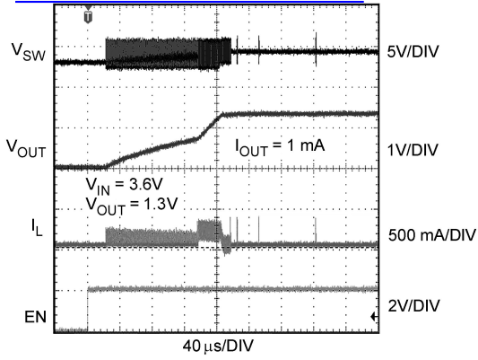
Start Up into PFM Mode V_{IN} = 3.6V ( V_{OUT} = 1.3V , Output Current = 1mA)
