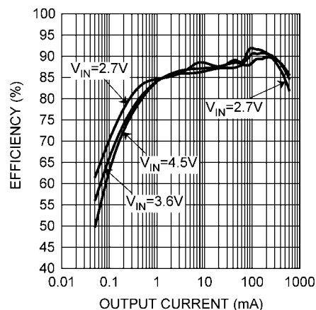
Efficiency vs. Output Current ( V_{OUT} = 1.8V )
