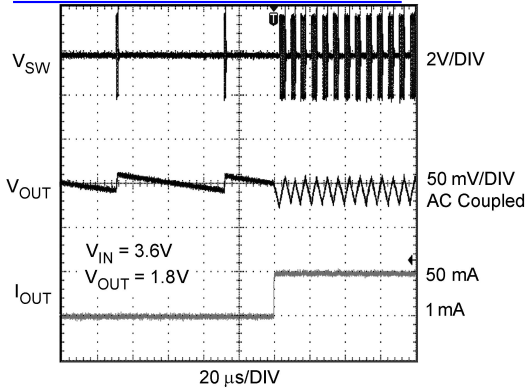
Load Transient Response ( V_{OUT} = 1.8V ) (PWM Mode 1mA to 50mA)
