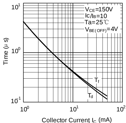
Turn-on switching times
