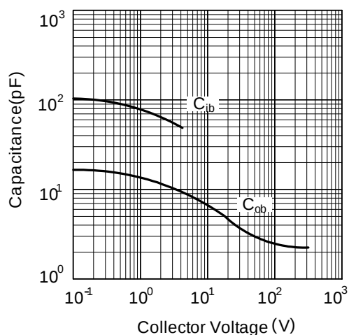
Capacitance
