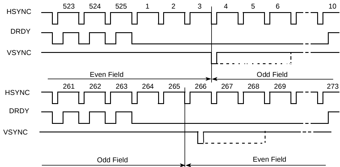
Line and Field Timing - NTSC
