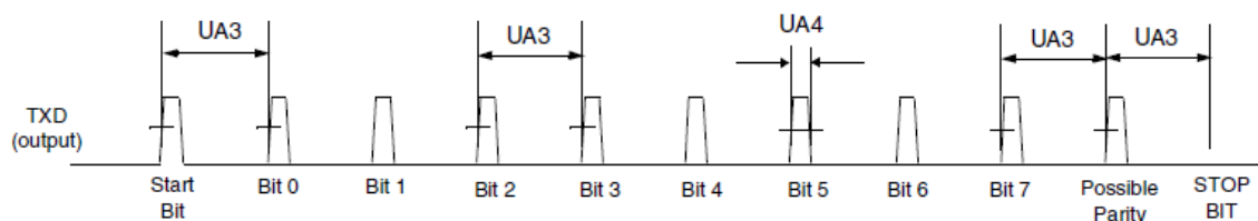
Figure 97. UART IrDA Mode Transmit Timing Diagram
