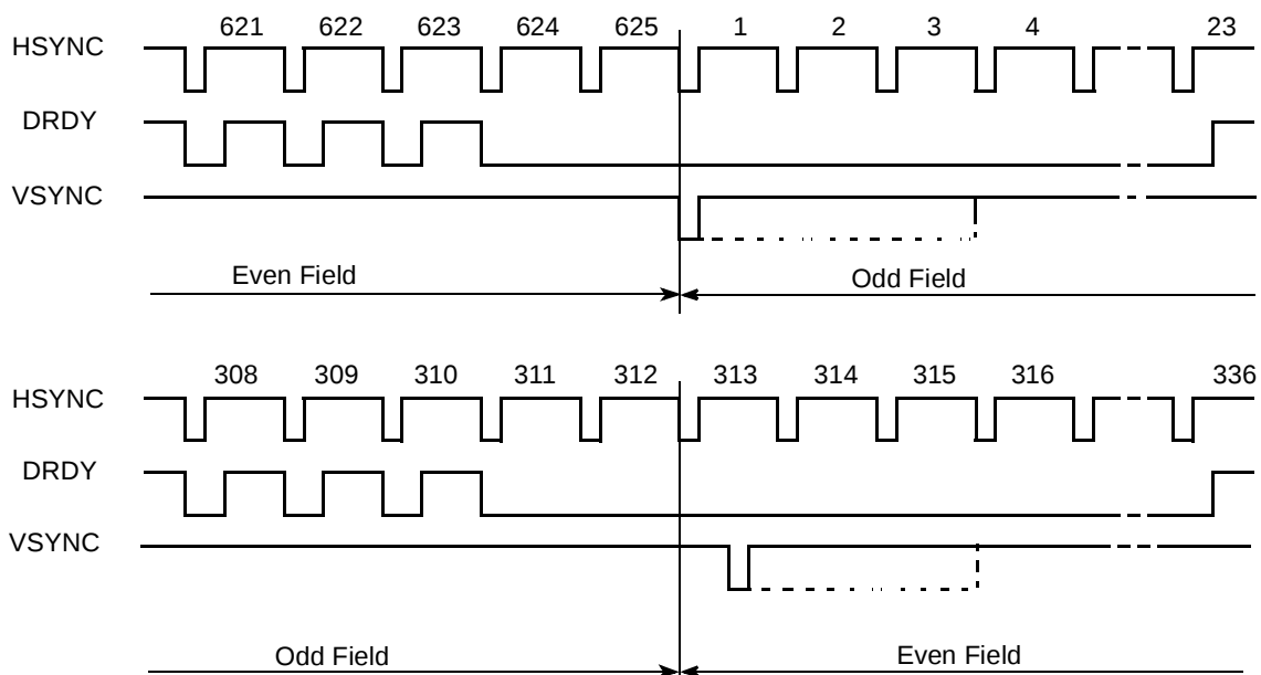
Line and Field Timing - PAL
