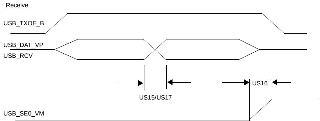
Figure 102. USB Receive Waveform in DAT_SE0 Uni-directional Mode
