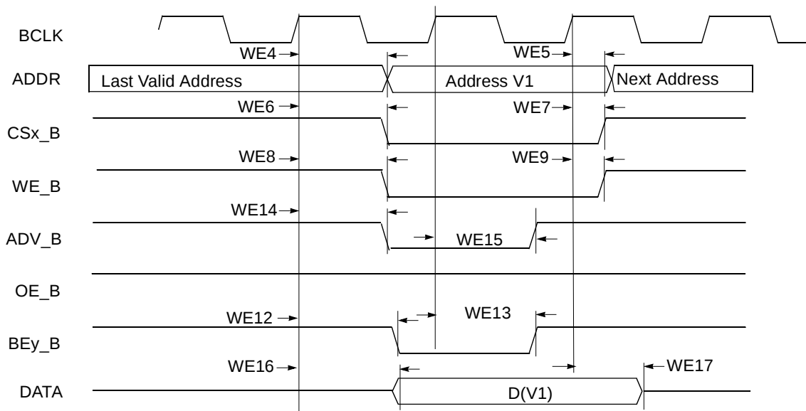
Figure 23. Synchronous Memory, Write Access, WSC=1, WBEA=1, WBEN=1, and WADV=0
