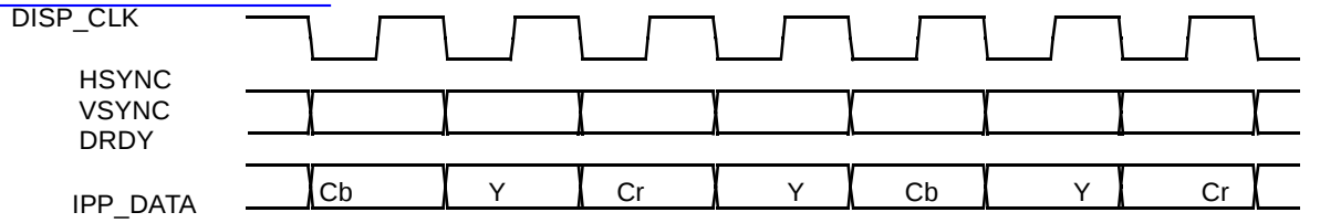
Pixel Data Timing
