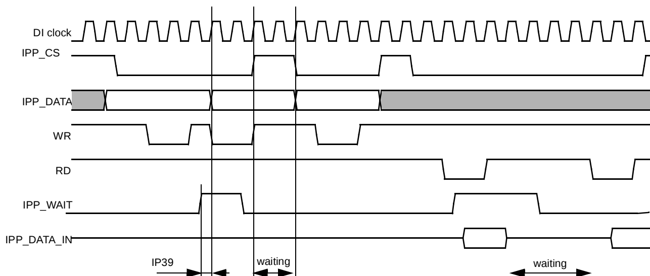
Figure 61. Parallel Interface Timing Diagram—Read Wait States
