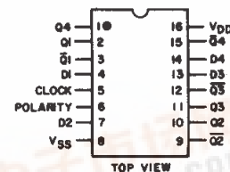
TERMINAL ASSIGNMENT
