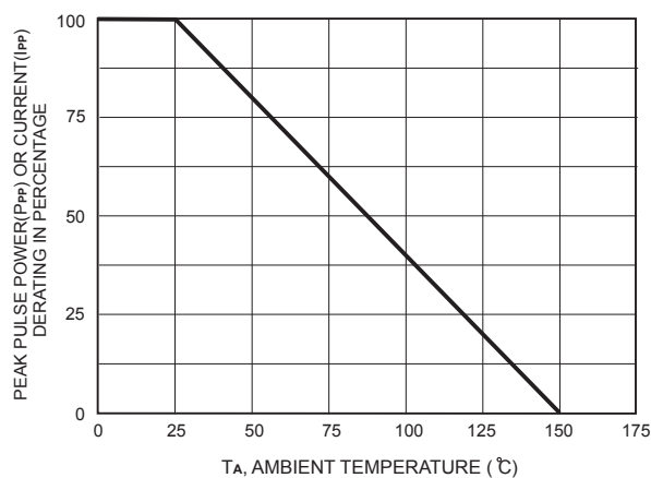
FIG.2-PULSE DERATING CURVE
