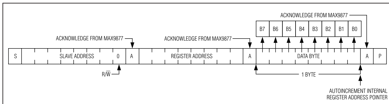
Figure 9. Writing One Byte of Data to the MAX9877
