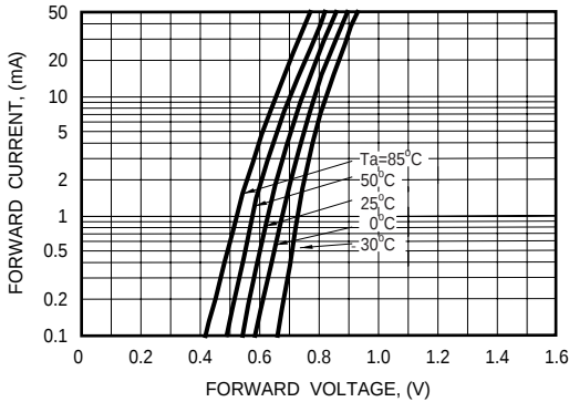
FIG. 2 - FORWARD CHARACTERISTICS
