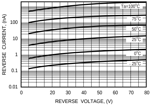
FIG. 4 - REVERSE CHARACTERISTICS
