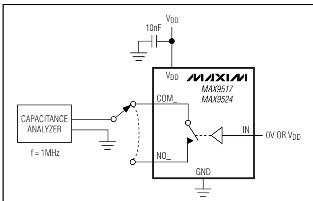
Figure 16. Channel Off-/On-Capacitance
