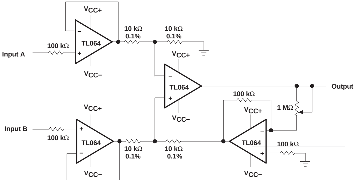
Figure 19. Instrumentation Amplifier
