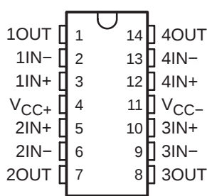
TL064 . . . D, J, N, NS, PW, OR W PACKAGE TL064A, TL064B . . . D OR N PACKAGE (TOP VIEW)
