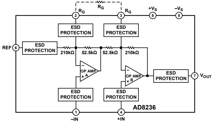
Figure 34. Simplified Schematic
