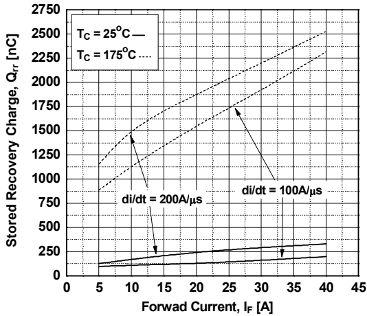
Figure 23. Stored Charge
