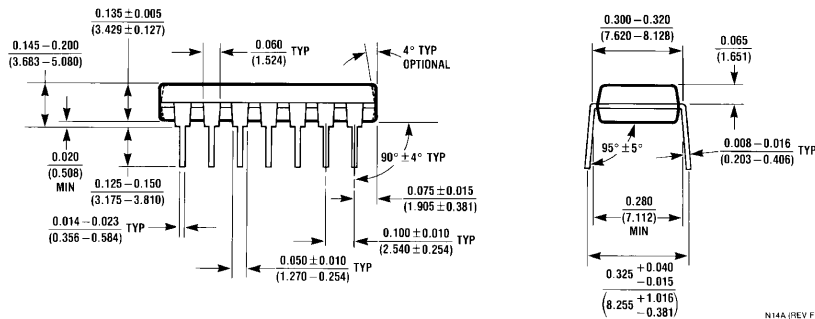
14-Lead Molded Dual-In-Line Package (N) Order Number DM74LS11N NS Package Number N14A
