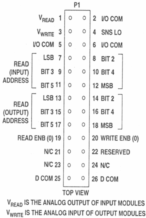
Figure 3 5B02 Pin-outs
