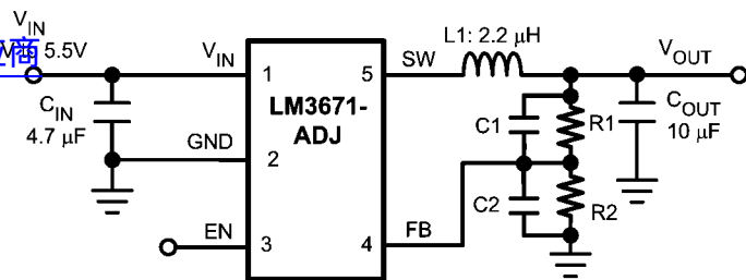
FIGURE 2. Typical Application Circuit for ADJ version
