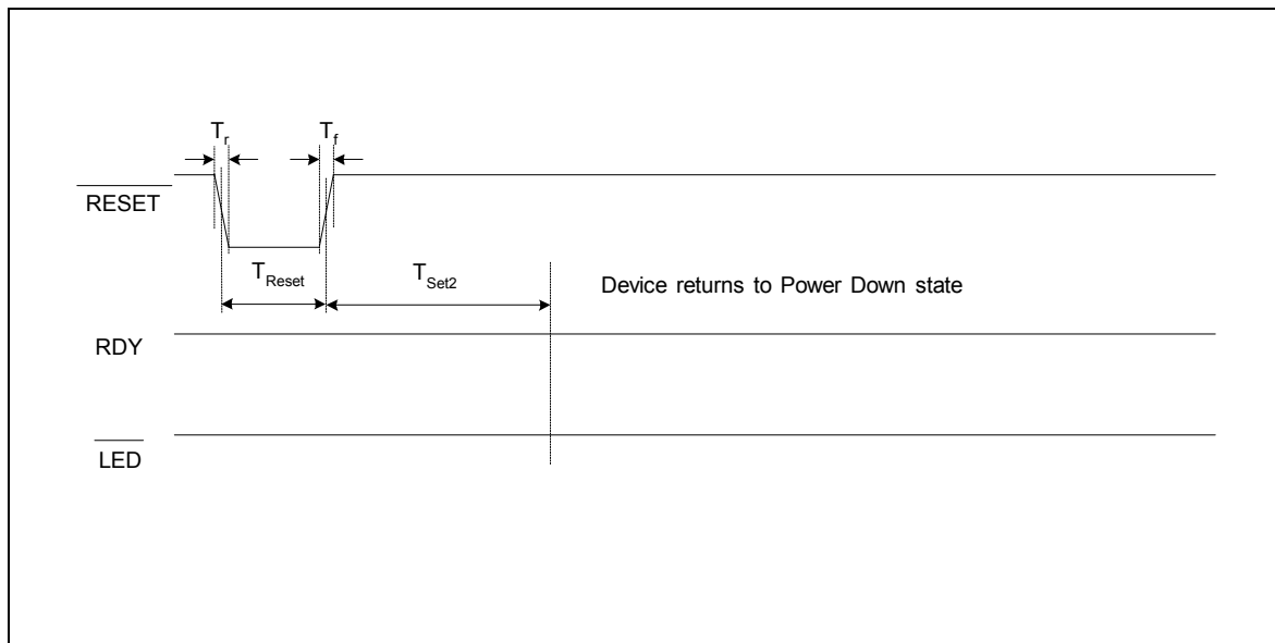
Figure 12.6: Reset Operation
