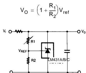
Figure 11. Shunt Regulator
