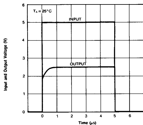
Figure 9. Pulse Response
