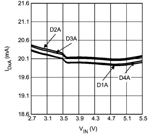
GroupA Current Matching vs Input Voltage 4 LEDs
