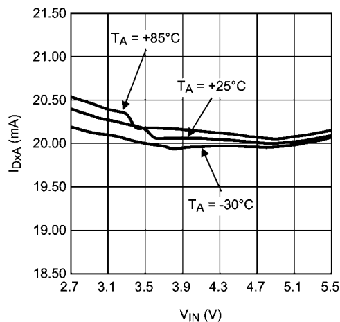
GroupA Diode Current vs Input Voltage
