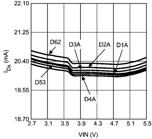
GroupA Current Matching vs Input Voltage 查询"LM2756TM"LEDs
