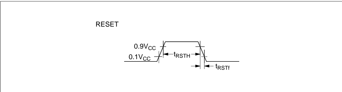
Figure 106 Reset Timing
