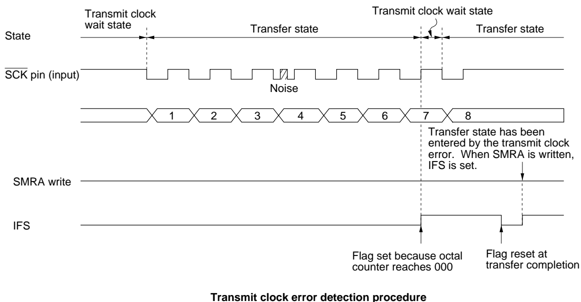
Figure 73 Transmit Clock Error Detection
