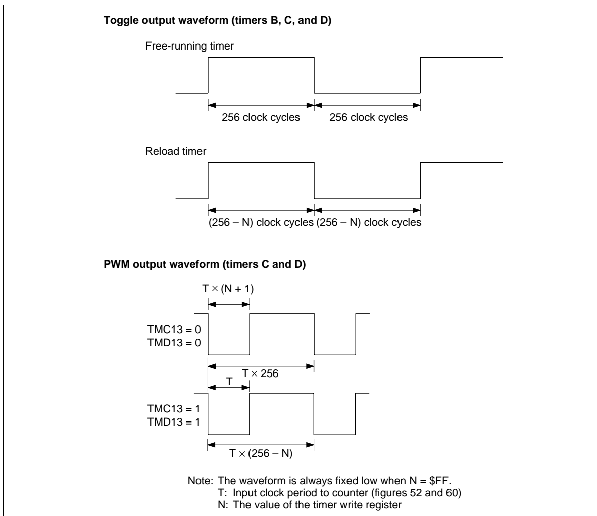
Figure 46 Timer Output Waveform
