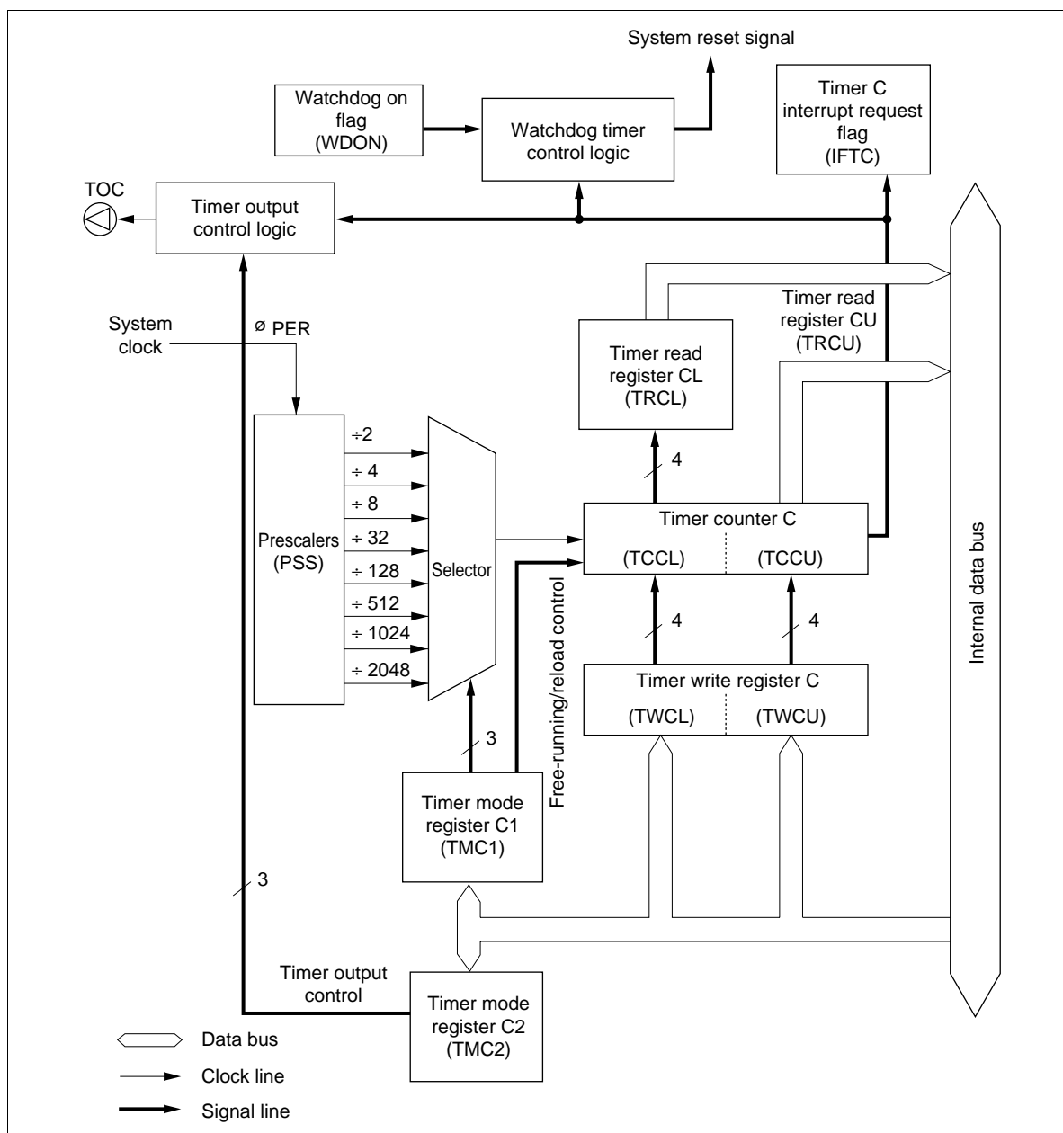
Figure 54 Block Diagram of Timer C
