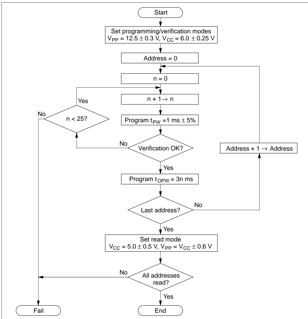
Figure 96 Flowchart of High-Speed Programming
