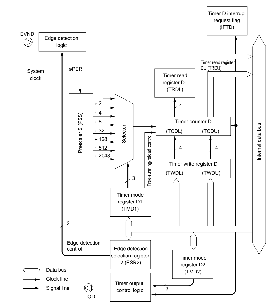
Figure 61 Block Diagram of Timer D (Free-Running/Reload Timer)
