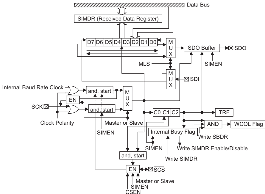
Block Diagram
