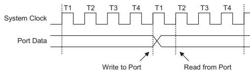
Read/Write Timing
