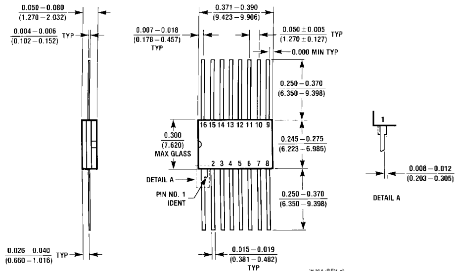
16-Lead Ceramic Flatpak (F) Package Number W16A
