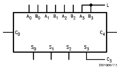
FIGURE 2. 3-Bit Adder
