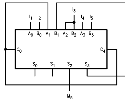
FIGURE 5. 5-Input Majority Gate
