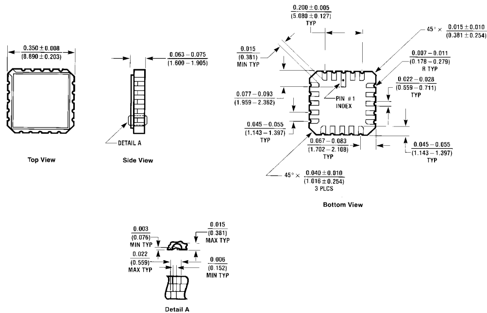
20-Lead Ceramic Leadless Chip Carrier (L) Package Number E20A
