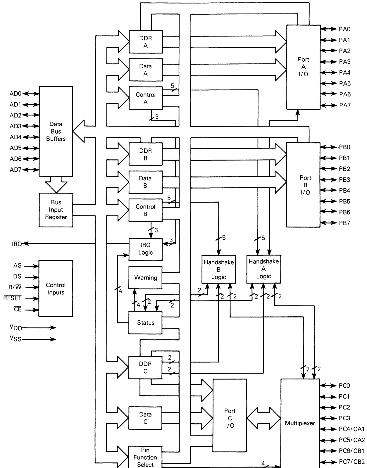
BLOCK DIAGRAM
