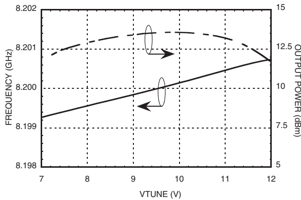
Frequency & Power vs. Tuning Voltage
