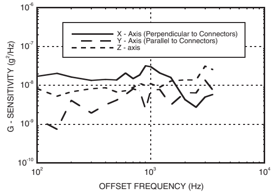
Vibration Sensitivity
