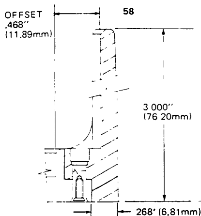
Offset Card Guides Factory Assembled with NO. 4-40 Threaded Insert
