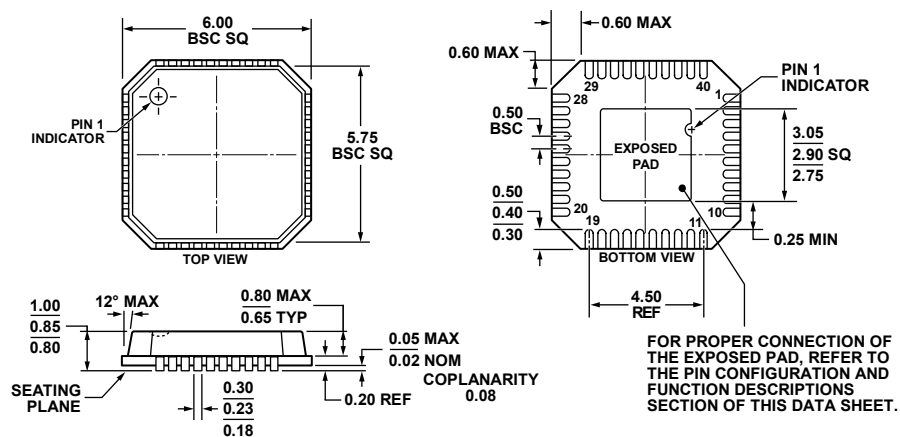
Figure 23. 40-Lead Lead Frame Chip Scale Package [LFSCP_VQ] 6 mm x 6 mm Body, Very Thin Quad (CP-40-8) Dimensions shown in millimeters
