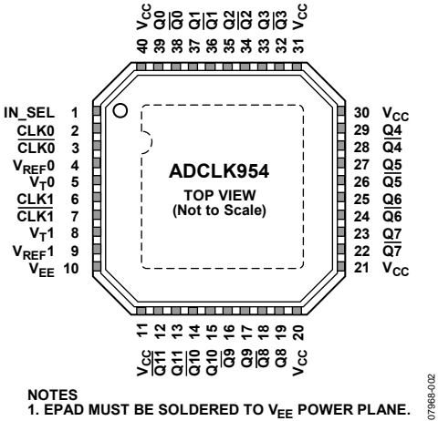
Figure 2. Pin Configuration
