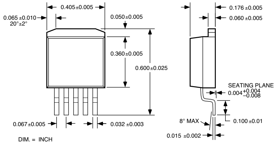
5-Lead TO-263 (T)
