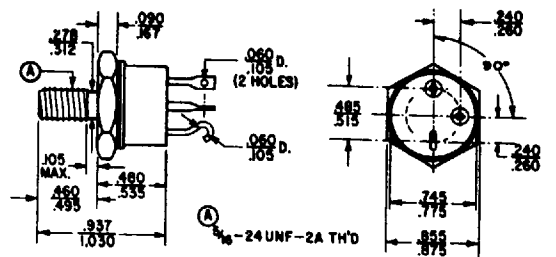
TO-63
