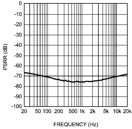
PSRR vs Frequency 查询"LM4995_07"中文资料 V_{DD} = 3V, R_L = 8\Omega
