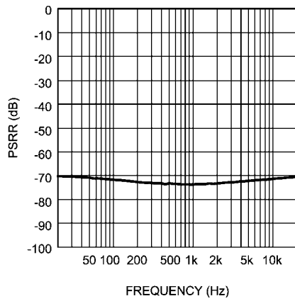
PSRR vs Frequency V_{DD} = 5V, R_L = 8\Omega
