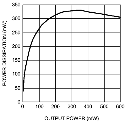
Power Dissipation vs Output Power V_{DD} = 3.6V, R_L = 8\Omega
