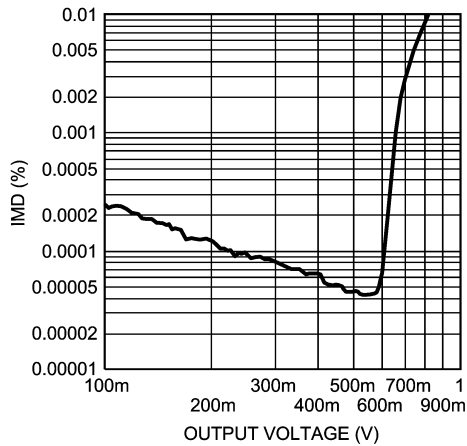
IMD vs Output Voltage
