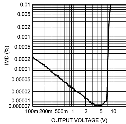
IMD vs Output Voltage
