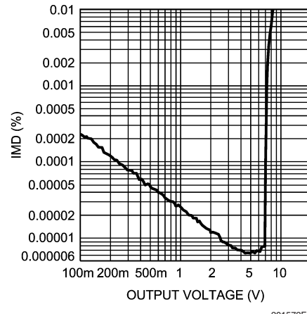
IMD vs Output Voltage
