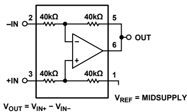
Figure 43. Difference Amplifier, Gain = 1, Referenced to Midsupply
