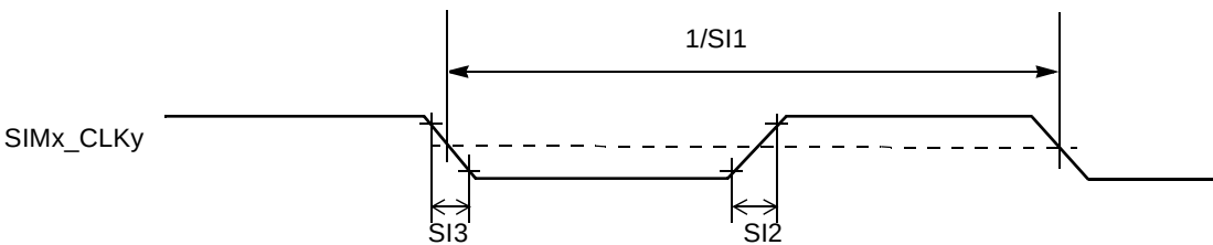
Figure 83. SIM Clock Timing Diagram
