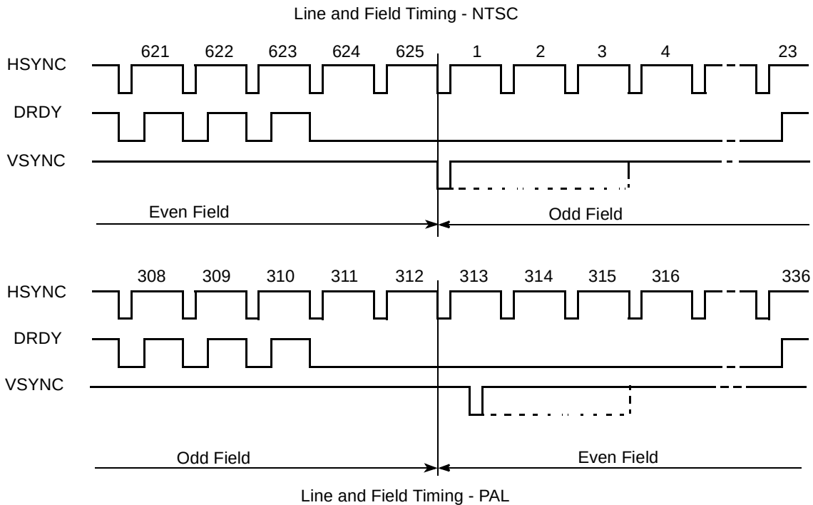
Figure 56. TV Encoder Interface Timing Diagram
