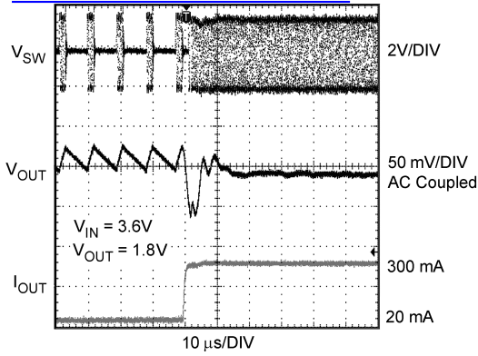
Mode Change by Load Transients V_{OUT} = 1.8V (PF to PWM)
