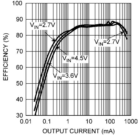
Efficiency vs. Output Current 查询"LM3677TL-1.3"供应商 (V_{OUT} = 1.3V)
