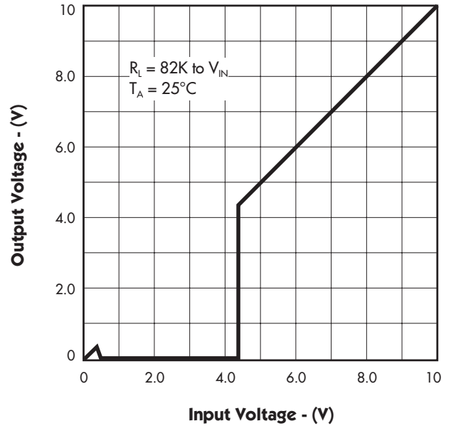
FIGURE 2. — \overline{RESET} OUTPUT VOLTAGE vs. INPUT VOLTAGE
