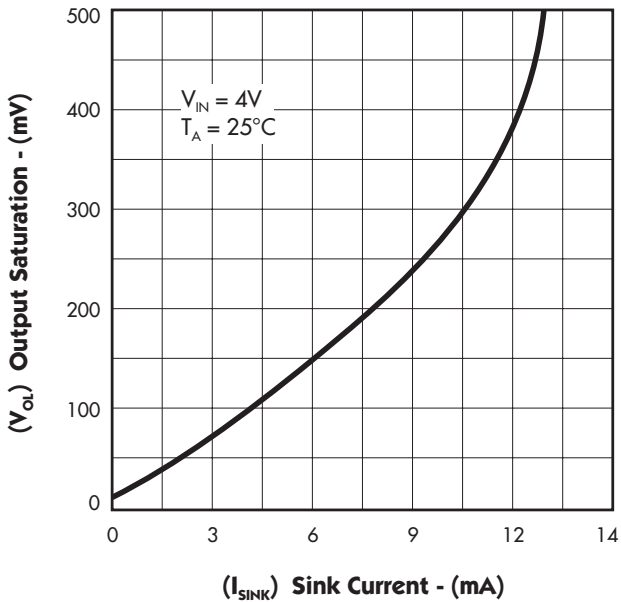
FIGURE 3. — \overline{RESET} OUTPUT SATURATION vs. SINK CURRENT
