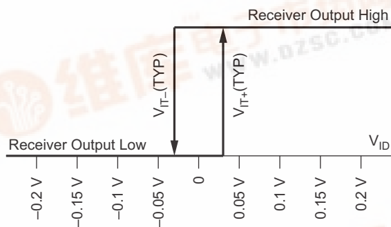
BALANCED RECEIVER INPUT THRESHOLDS
