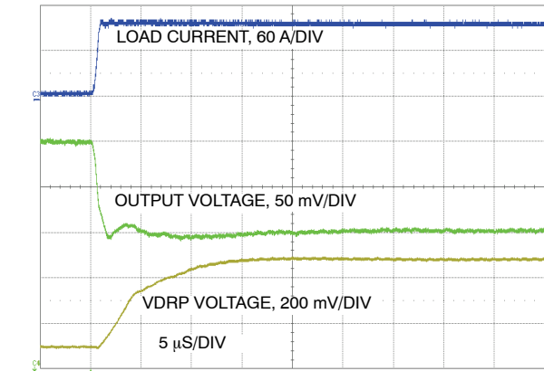
Figure 32. Output Voltage – 1.2\text{ nF} Capacitor in Parallel with R_{DRP}
