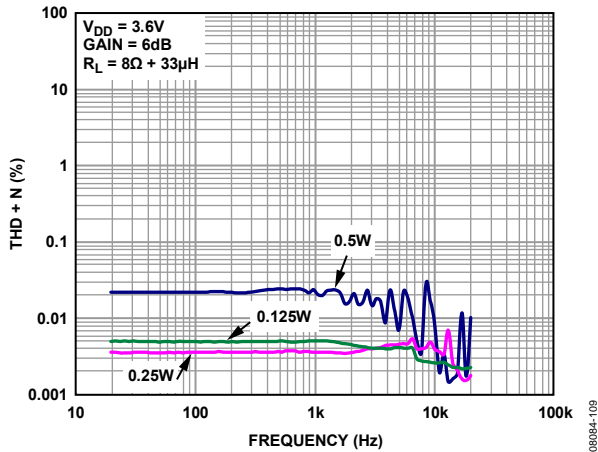
Figure 11. THD + N vs. Frequency, V_{DD} = 3.6V , R_L = 8\Omega , A_v = 6dB
