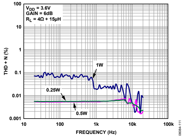
Figure 13. THD + N vs. Frequency, V_{DD} = 3.6V , R_L = 4\Omega , A_v = 6dB
