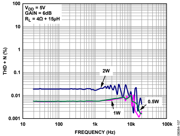
Figure 9. THD + N vs. Frequency, V_{DD} = 5V , R_L = 4\Omega , A_v = 6dB
