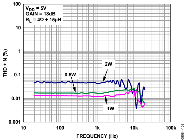
Figure 10. THD + N vs. Frequency, V_{DD} = 5V , R_L = 8\Omega , A_v = 18dB
