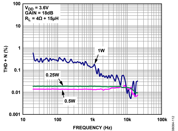
Figure 14. THD + N vs. Frequency, V_{DD} = 3.6V , R_L = 4\Omega , A_v = 18dB
