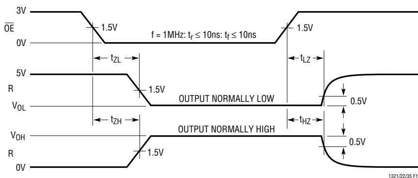
Figure 12. Receiver Enable and Disable Times
